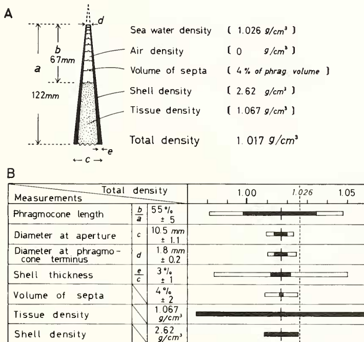
TEXT-FIG. 3. Calculation and error estimation of total density of Eubostyrioceras muramotoi Matsumoto, WEA 003T-1. A, estimated physical values. B, estimated error range for each value. Black rectangles show the fluctuation range of total average density when each value is 5% over- or underestimated. White rectangles show the fluctuation range as estimated from each measuring error.
